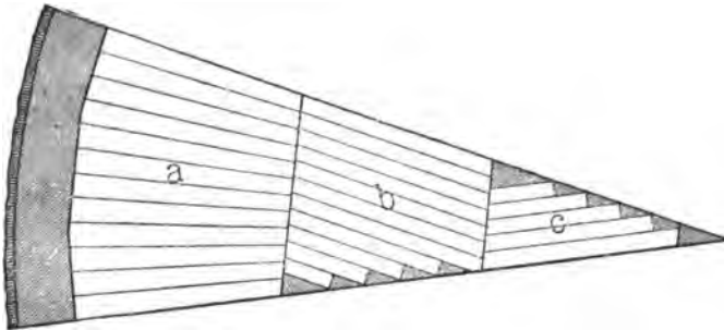
Fig. 338.—Method of splitting wood for cask staves. (After Boppe.)
